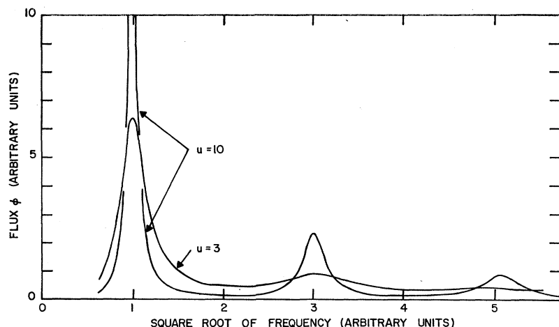
FIG. 1. Resonance curves for an infinite plate parallel to the x, y plane, with \alpha=0 . The frequency scales have been adjusted to bring the first peaks into coincidence (courtesy of M. T. Taylor).
